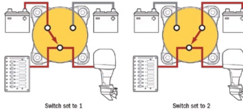
Switches isolated battery banks to all loads
