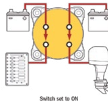
Simultaneously switches two isolated battery banks
